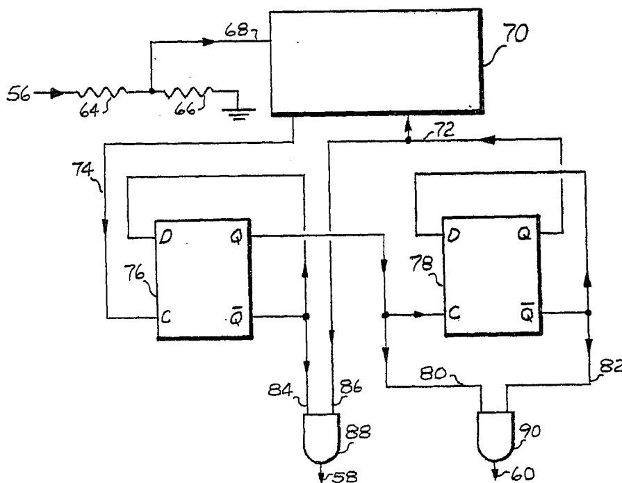
FIGURE 4. TIME WINDOW GENERATOR 32
